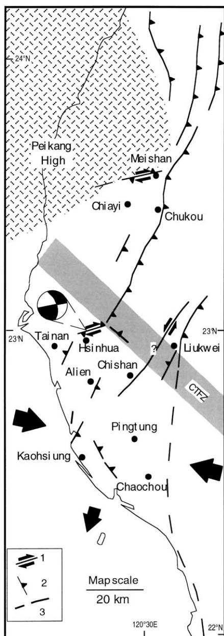
Fig. 8. Active faults in SW Taiwan (modified after Hsu and Chang, 1979). 1 — Active right-lateral/reverse motion along Meishan and Hsinhua faults and left-lateral motion along the Chishan fault. 2 — Active reverse fault motions. 3 — Inferred active fault. The large convergent black arrows indicate the average direction of shortening, the small arrow the subperpendicular direction of escape.
