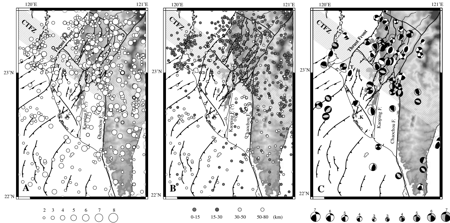
Fig. 2. Seismicity in southern Taiwan over the years 1900–1998 (source: Central Weather Bureau, Taiwan; USGS; CMT Harvard). (A) Earthquake distribution as a function of magnitude. Note the low seismicity and the low earthquake magnitude in SW Taiwan. (B) Earthquake distribution as a function of focus depth. North of the Chishan Transfer Fault Zone (CTFZ, hatched area), 0–30 km depth foci are numerous and related to actual collisional setting; south of the CTFZ, most earthquakes occur at depth larger than 25 km, which suggests that the upper crust, comprising the sedimentary wedge, mainly deforms by aseismic creep. (C) Earthquake focal mechanisms (dilatational first motion quadrants in white: after Rau and Wu (1998) for magnitudes lower than five; after Harvard for magnitudes larger than five; dilatational first motion quadrants in grey: after Yeh et al. (1991).
