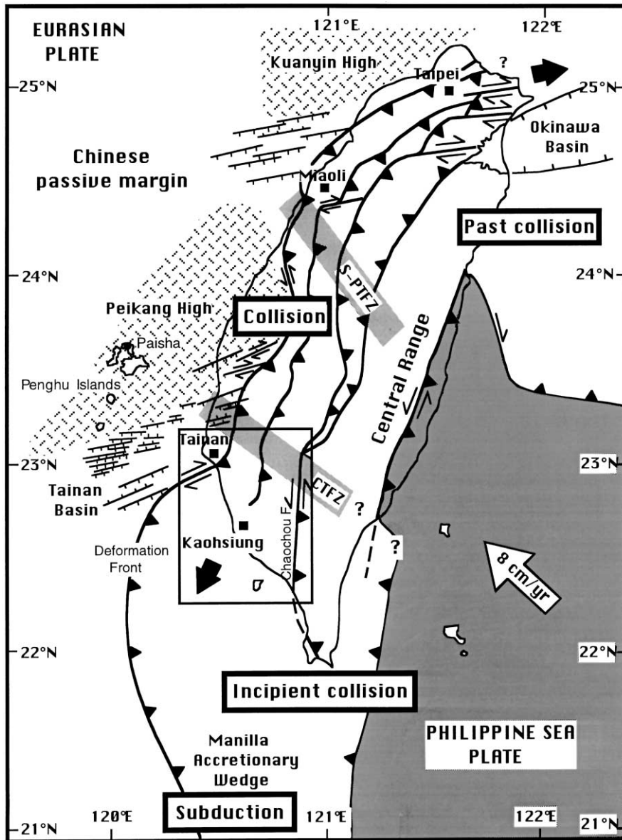
Fig. 1. Geotectonic setting and main structural features of Taiwan. The large open arrow shows the present direction of convergence of the Philippine Sea plate (dark grey) relative to South China; velocity after Yu et al. (1997, 1999). Heavy lines indicate major thrusts, triangles on upthrown side; lines with double arrows indicate major wrench faults. Hatched areas correspond to basement highs of the Chinese margin which underlie the deposits of the foreland basin which underlie the deposits of the foreland basin. Large black arrows indicate tectonic escape at the tips of the belt. The frame shows the location of the area investigated.
