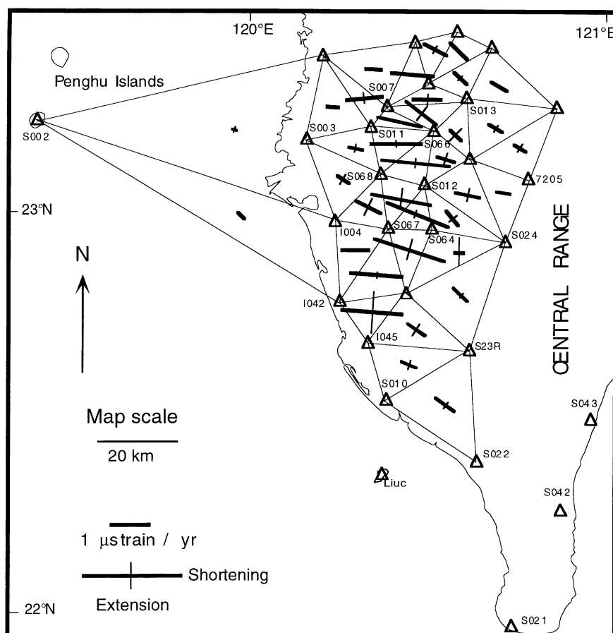
Fig. 5. Principal strain rates within GPS subnets in southwestern Taiwan (Yu and Chen, 1998). Heavy lines: strain axes in the area investigated, length proportional to magnitude (see scale).
