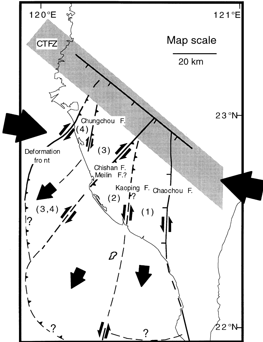
Fig. 11. Tentative model of escaping blocks in SW Taiwan. Arrows along the faults indicate the sense of along-strike component of motion. Note the inferred normal component of motion along the CTFZ.
