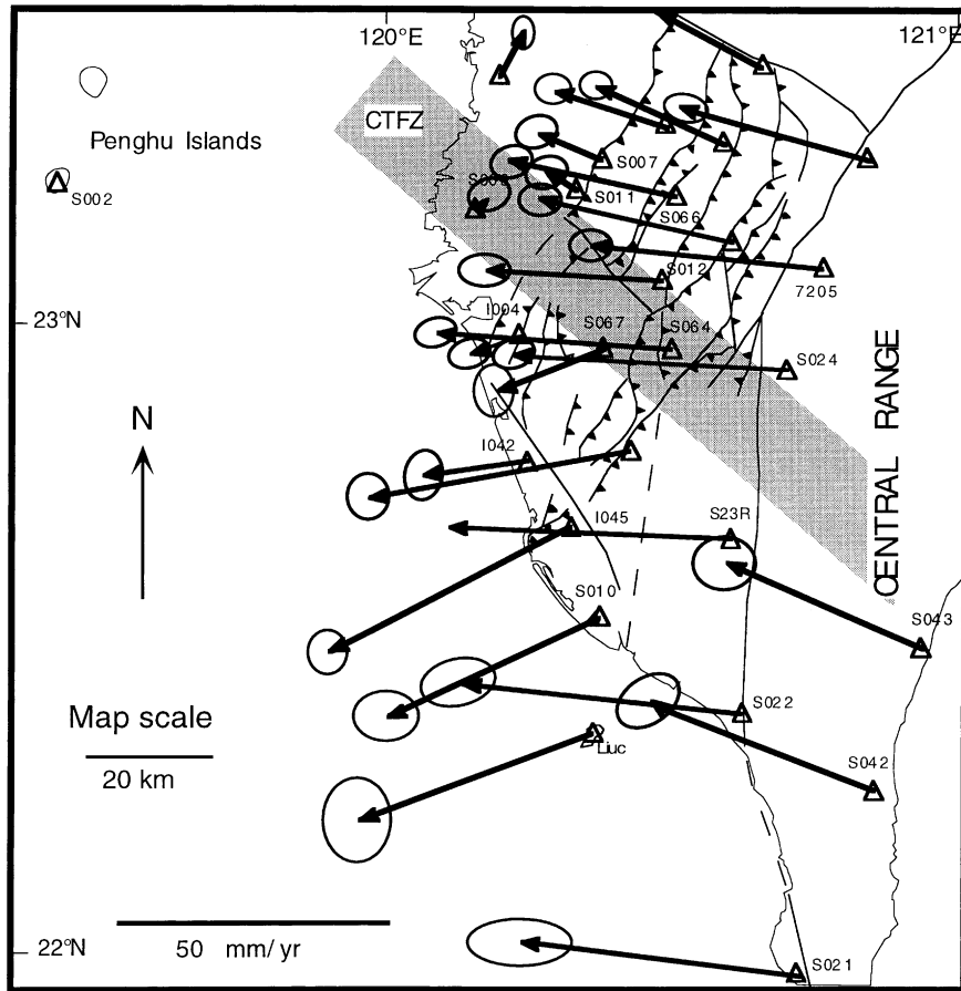
Fig. 4. GPS displacement velocity field in the area investigated (Yu et al., 1997), relative to Paisha (Penghu islands, see Fig. 1). Triangles: GPS stations. Black arrows connected to triangles: displacement vectors, length proportional to velocity. The 95% confidence ellipse is shown at the tip of each velocity vector. Note the southwestward present-day displacement south of the CTFZ, suggesting tectonic escape.
