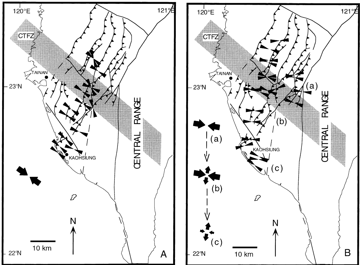
Fig. 9. Pleistocene stress patterns in southwestern Taiwan. (A) Pleistocene NW–SE compression. Convergent arrows indicate directions of \sigma_1 (data after Rocher et al., 1996; Mouthereau et al., 1998; Lacombe et al., 1999). The large black convergent arrows indicate the average regional compression. (B) Late (?) Pleistocene WNW–ESE to E–W compression. Note the along-strike change in the relative stress magnitudes (convergent arrows: compression, divergent arrows: extension) accompanying the regional E–W regional compression (a–c).
