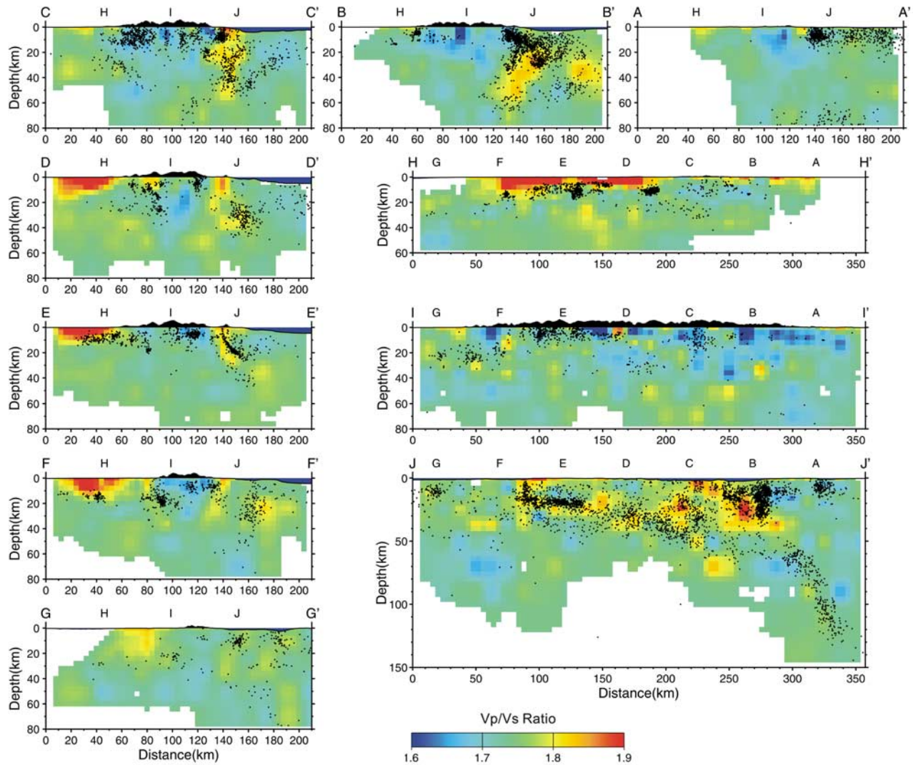
Figure 6b. V_p/V_s ratio profiles. The dots show the relocated events for M > 3 within \pm 5 km of each profile. Locations of the profiles A-A' to J-J' are indicated in Figure 2.
