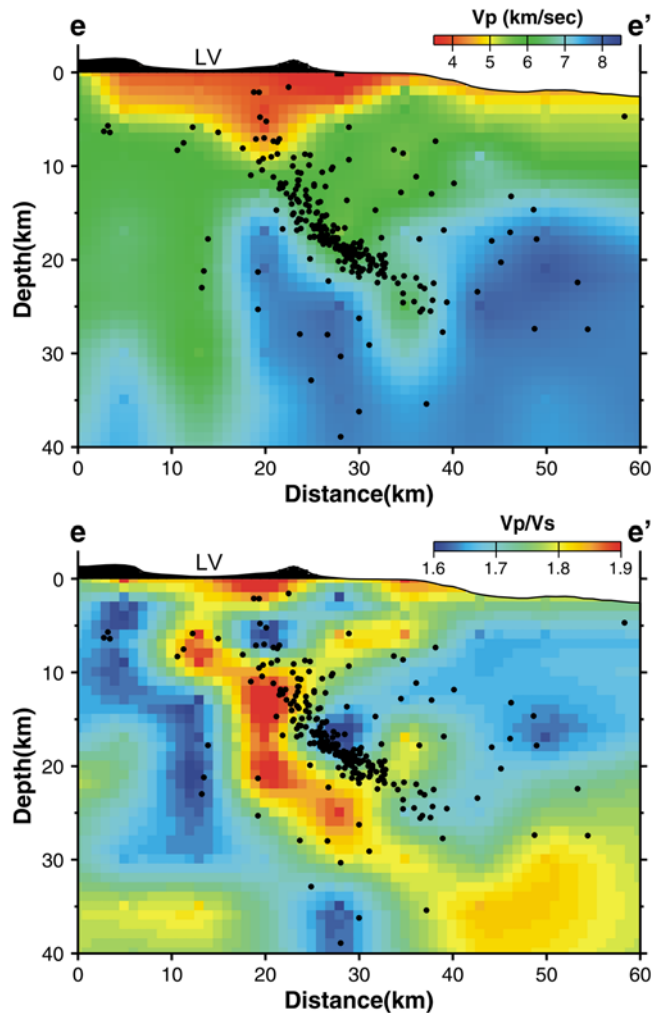
Figure 8. V_p velocity and V_p/V_s ratio profiles in eastern Taiwan. The dots show the relocated events for M > 3 within \pm 5 km of each profile. Location for the e-e' profile is shown in Figure 2. LV marks the location of Longitudinal Valley.
