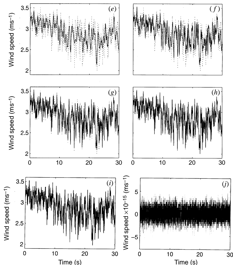
Figure 7. Cont. (e) Data (in the dotted line) and the sum of c_9-c_5 components (in the solid line). (f) Data (in the dotted line) and the sum of c_9-c_4 components (in the solid line). (g) Data (in the dotted line) and the sum of c_9-c_3 components (in the solid line). By now, we seem to have recovered all the energy containing eddies. (h) Data (in the dotted line) and the sum of c_9-c_2 components (in the solid line). (i) Data (in the dotted line) and the sum of c_9-c_1 components (in the solid line). This is the final reconstruction of the data from the IMFs. It appears no different from the original data. (j) The difference between the original data and the reconstructed one; the difference is the limit of the computational precision of the personal computer (PC) used.
