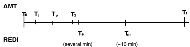
Figure 9. Timing of event occurrence at T_0 , P -wave arrival at T_1 , grid search for location and MT determination starting at T_2 and completing at T_3 in the AMT system, and an event notification arrival by e-mail at T_e and MT determination at T_{mt} in the REDI system. T_t illustrates tsunami arrival time for an epicentral distance of about 200 km.
