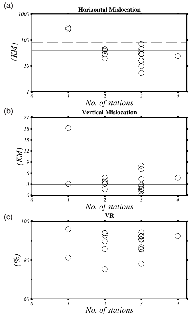
Figure 8. Effects of the number of stations on the inversion results using the onshore events. (a) The horizontal mislocation; (b) the vertical mislocation; (c) the maximum variance reduction VR. Q1 solutions are plotted below the solid line, Q3 solutions above the dashed line, and Q2 solutions are in between.
