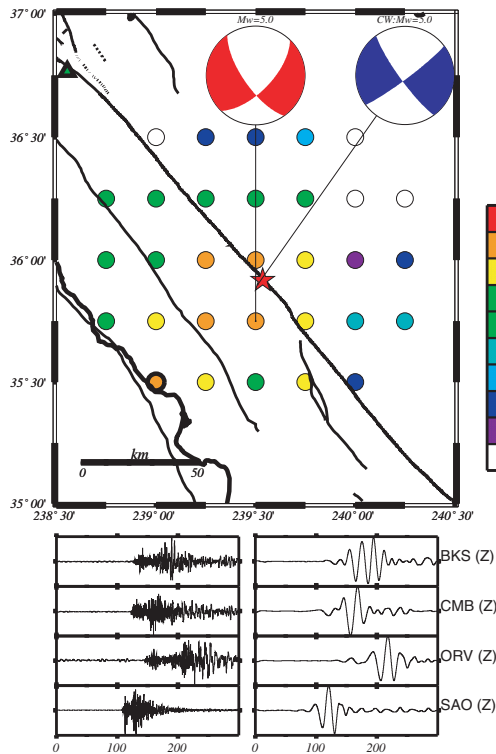
Figure 4. Snapshots of the AMT simulation for the 20 December 1994 Parkfield event ( M_L 4.7, origin time 10:27:48). Waveforms in the 5-min window that is shifted every 20 sec are inverted for all the grid points (color coded to show the level of VR) from 10:24:00.00 to 10:34:00.00. The AMT solution is shown with a red beach ball, and the REDI solution is shown with a blue beach ball at the red star. (a) Source signals barely enter the window where the maximum (VR = 31.9%); (b) much of the source signals are included in this time window (VR = 90.5%; t_0 = 10:26:20); (c) AMT inversion performed over a finer grid ( \Delta x \sim 0.25^\circ ) in a smaller area around the detected location (VR = 92.1%; t_0 = 10:26:20); and (d) the front part of the seismic wavetrain is outside of the window (VR = 65.8%; t_0 = 10:29:00) (see the text for details).
