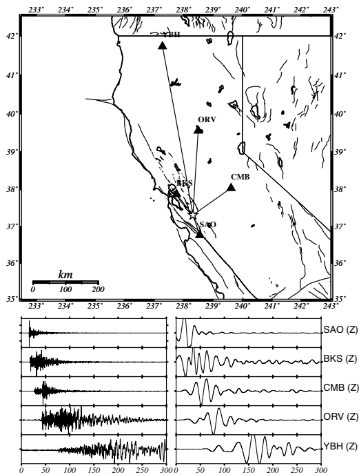
Figure 3. (Top) Source and station location paths for the 11 August 1993 San Felipe earthquake ( M_L 4.6). (Bottom left) Raw waveforms and (bottom right) waveforms filtered in the 20–50 mHz band.
