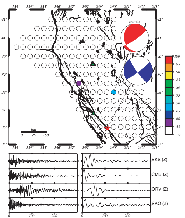
Figure 4. Snapshots of the AMT simulation for the 20 December 1994 Parkfield event ( M_L 4.7, origin time 10:27:48). Waveforms in the 5-min window that is shifted every 20 sec are inverted for all the grid points (color coded to show the level of VR) from 10:24:00.00 to 10:34:00.00. The AMT solution is shown with a red beach ball, and the REDI solution is shown with a blue beach ball at the red star. (a) Source signals barely enter the window where the maximum (VR = 31.9%); (b) much of the source signals are included in this time window (VR = 90.5%; t_0 = 10:26:20); (c) AMT inversion performed over a finer grid ( \Delta x \sim 0.25^\circ ) in a smaller area around the detected location (VR = 92.1%; t_0 = 10:26:20); and (d) the front part of the seismic wavetrain is outside of the window (VR = 65.8%; t_0 = 10:29:00) (see the text for details).
