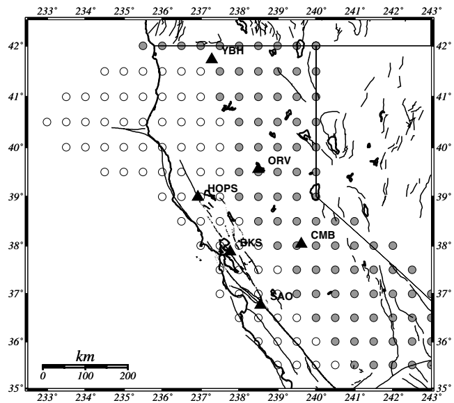
Figure 2. Virtual source points (shown with 160 small circles) on the grid and station locations (triangles). The source locations are distinguished between the models: open circles for GIL7 and shaded circles for SoCal.
