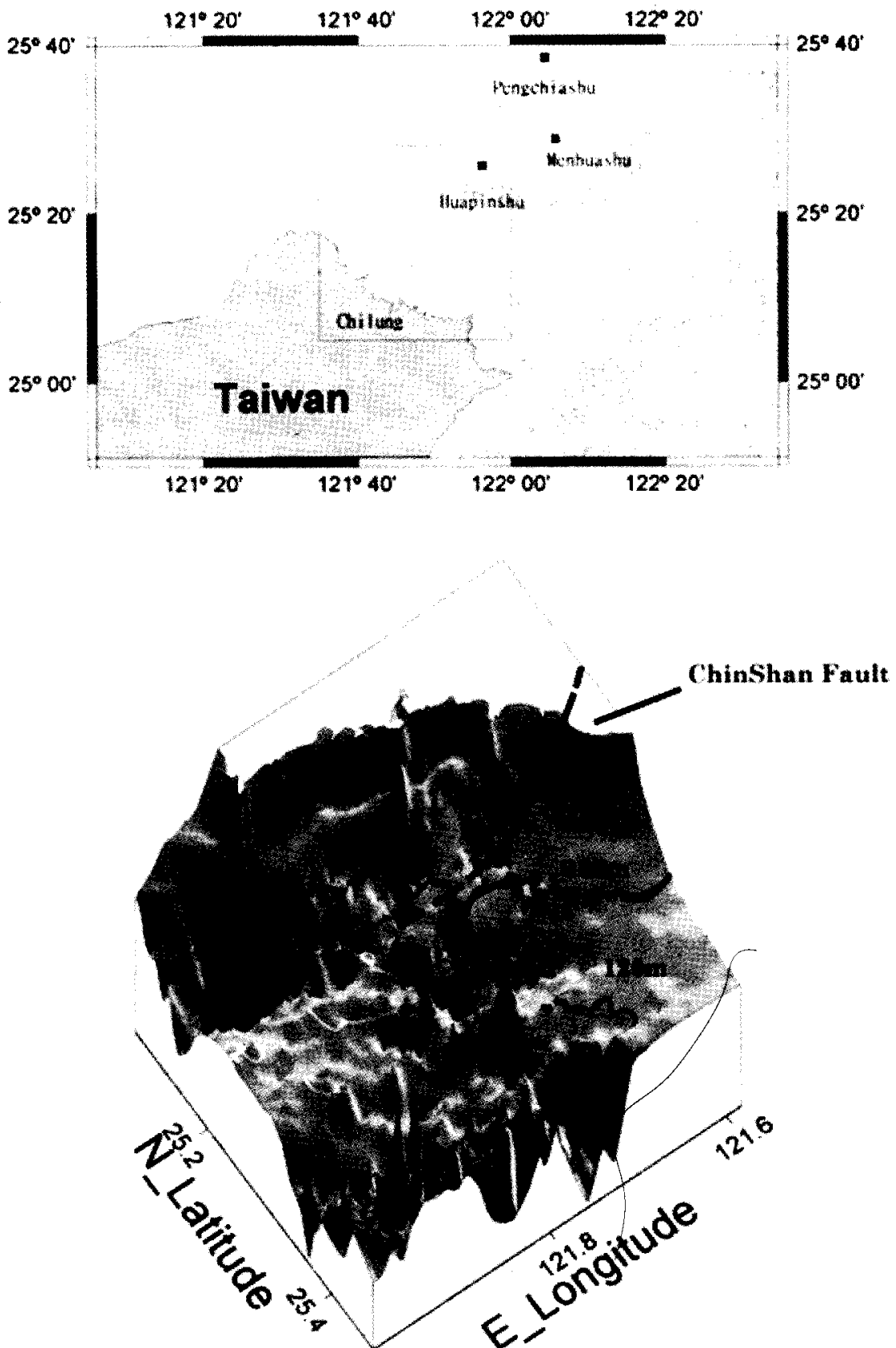
Fig. 8. 3-D plot around the west end of the Chilung Shelf. The 100m and 120m isobaths are shown by solid black lines, while the 140m isobath is shown by the white line. The dash line represents the possible path of the Chinshen Fault under the ocean.
