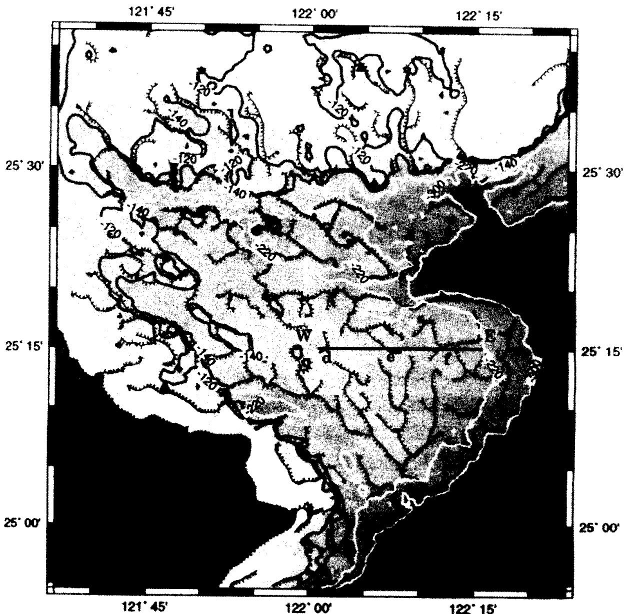
Fig. 5. Map showing 120, 140, 220 and 300m isobaths indicating the traces of the inner and the outer shelf breaks. The E-W straight line is the location trace of the seismic profile shown in Figure 9. d, e and f mark the targets found along the profile intersecting with the “break” lines. The “break” lines are done by the self-developed automatic line extraction computer program (Chang, 1997). These “break” lines indicate the edge traces of the break topography as discussed in the text.
