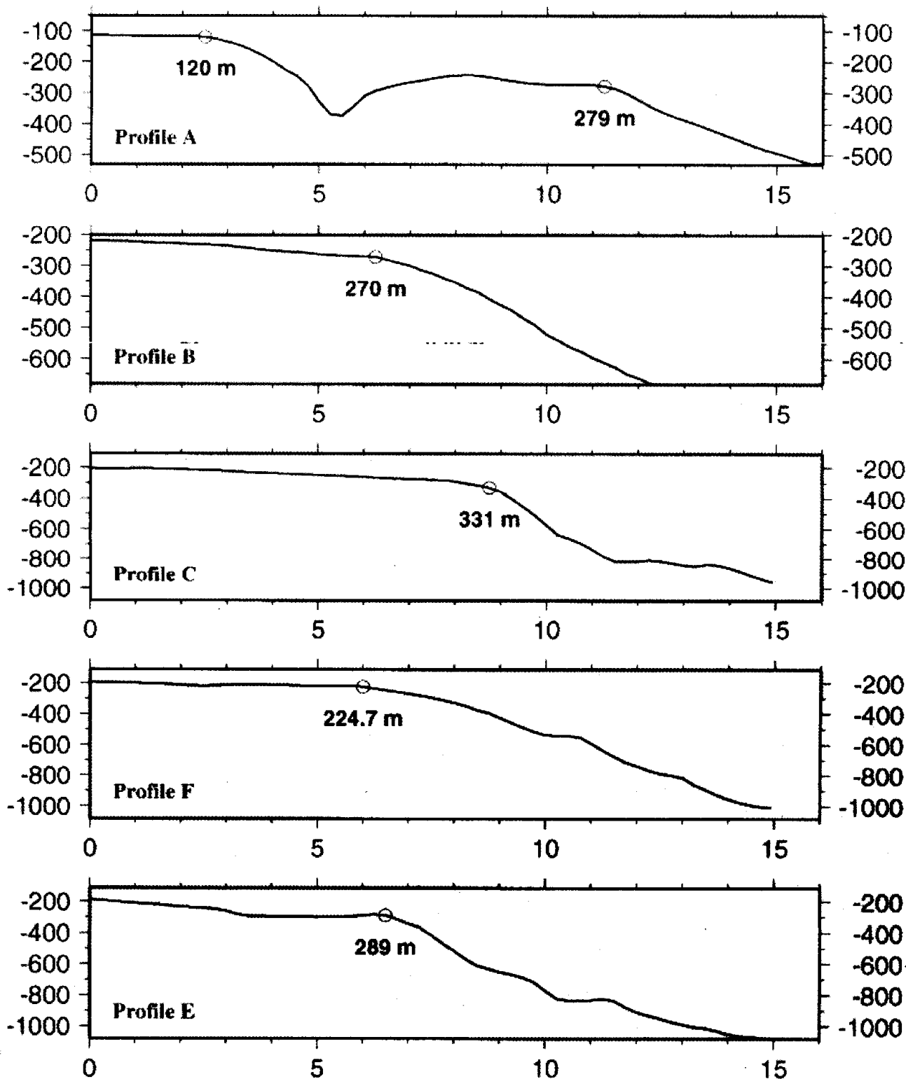
Fig. 11. Five profiles denoting the depths of the breaks across the shelves. The locations of the profiles are shown in Figure 10. The X axes represent the horizontal distances in kilometers, while the Y axes are the water depths in meters. The locations of the shelf break determined numerically (Chang, 1997) are marked by open circles.
