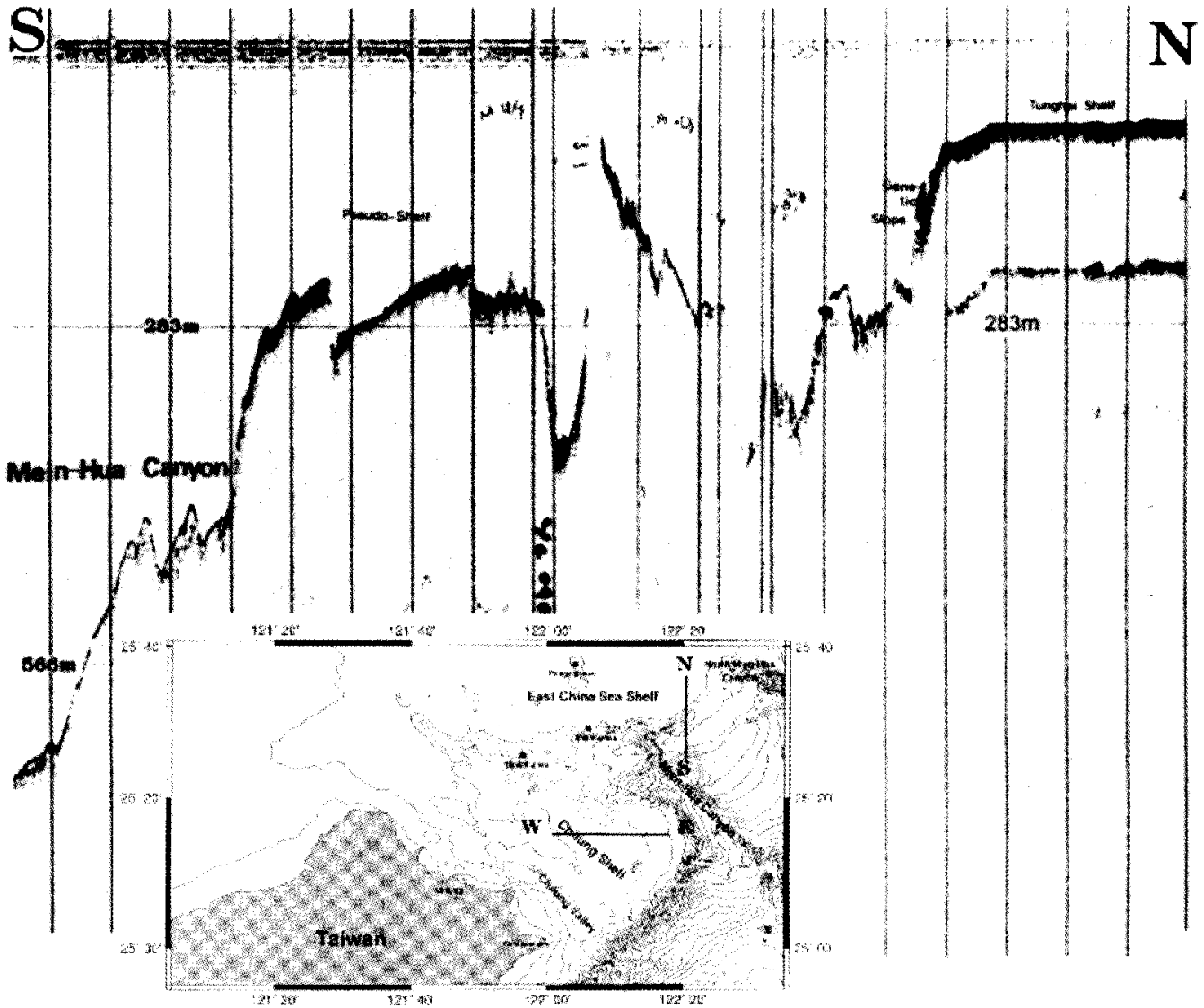
Fig. 14. 3.5kHz profile across the CLPS area. This subbottom profiler data set was obtained on the 348 cruise of the R/V OR-I. The profile shows normal faulted behavior with subsided blocks on/toward the flank of the pseudo-slope (Song et al. , 1997). Location map of the profile (denoted by S-N) is in the lower-left hand corner.
