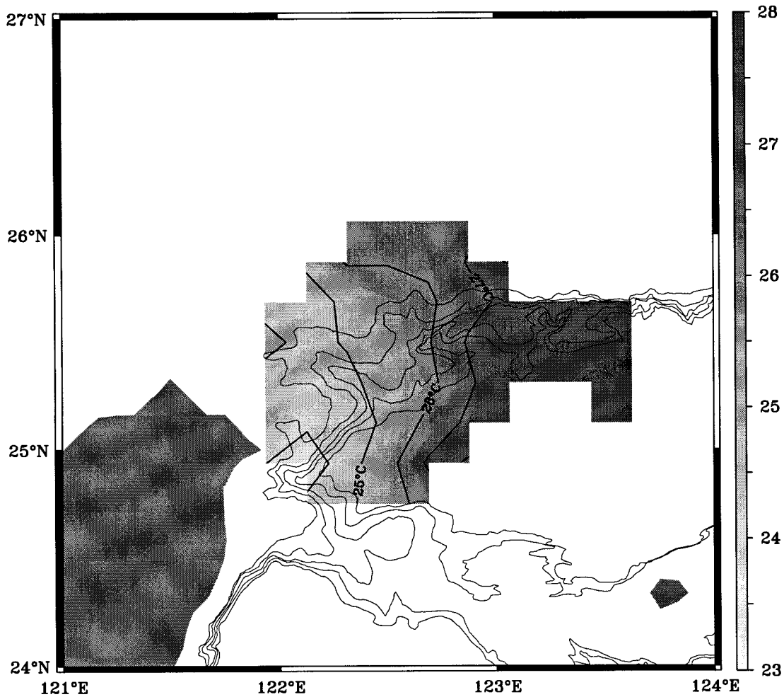
FIG. 7. Temperature distribution at 16 m from the hydrographic survey conducted during 10–17 August 1994. The temperature is contoured at intervals of 1°C. The depth contours are thin.
