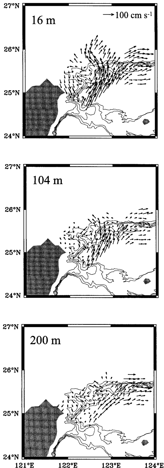
FIG. 2. Phase-averaged current vectors from SADCP observations at depth (a) 16, (b) 104, and (c) 200 m. The bathymetry is shown with thin depth contours from 200 to 1000 m at intervals of 200 m.
