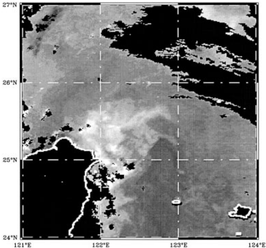
FIG. 6. Infrared image of the sea surface temperature in the study area obtained by NOAA-11 on 12 August 1994. Light shading indicates low surface temperature.
