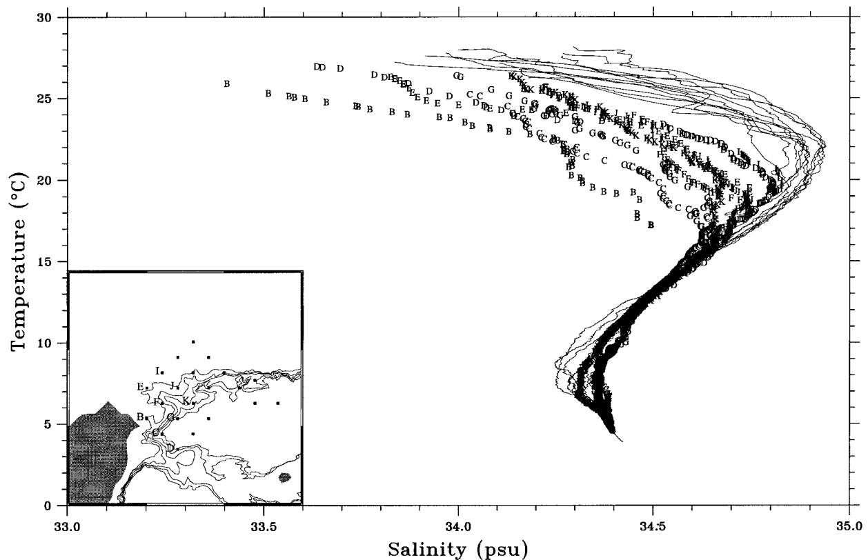
FIG. 8. Temperature-salinity plot of all the hydrographic station data from the survey during 10–17 August 1994. The solid curves represent T - S associations found at stations in the Kuroshio. The T - S associations found at stations, of which the station letters are shown in the locator map inset, are represented with strings of the station letters.
