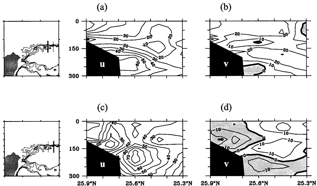
FIG. 5. Vertical sections of (a) eastward and (b) northward velocity components along the track connecting stations U and W and of (c) eastward and (d) northward velocity components along the track connecting stations X and Z. The depth range is from the surface to about 300 m. The continental shelf is darkened. The values are contoured at intervals of 10 \text{ cm s}^{-1} . The zero contour is shown in heavy line. Portions of negative values are shaded.
