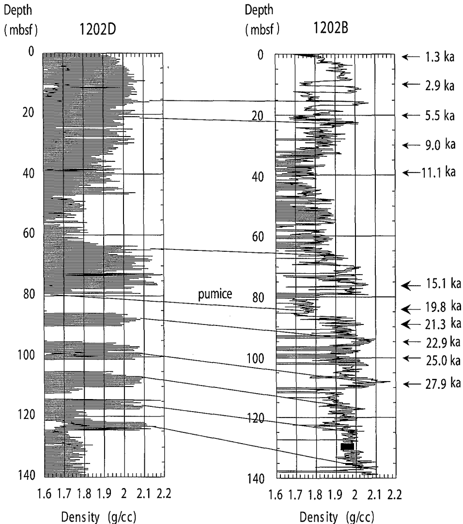
Fig. 4. Correlation between ODP Holes 1202B and 1202D based upon characteristics of bulk density measured by the GRA densiometer of the Multi-Sensor Track (MST) system on board Leg 195 (Shipboard Scientific party 2002). The pumice layer serves as a benchmark marker. Also marked are Carbon-14 dates in thousand years (ka) of calendar age for Hole B.
