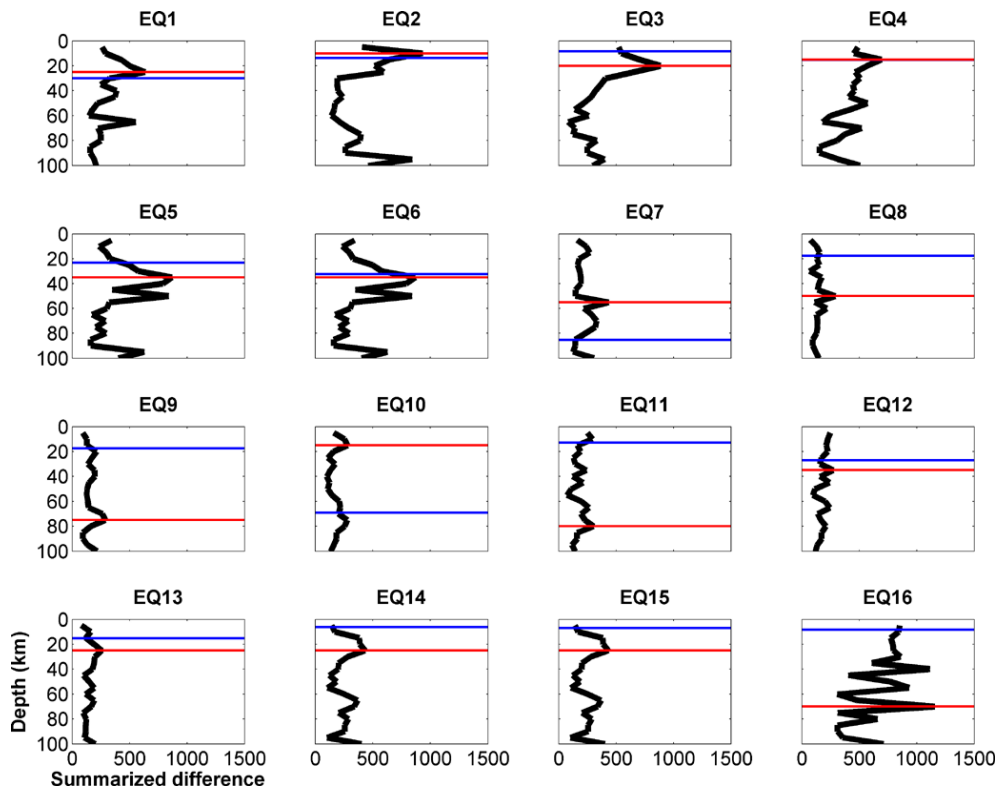
Fig. 5. The computed and reported hypocentre depths of 16 earthquakes. The blue lines denote reported hypocentre depths. The black lines show summarised differences on the depth profile. The red lines are the computed depths determined by the largest summarised differences.
