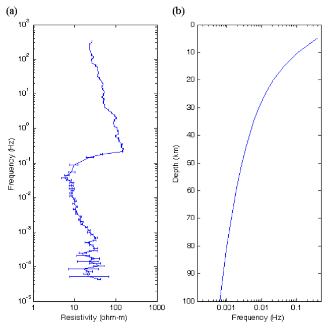
Fig. 2. The apparent resistivity of magnetotelluric data (retrieved from Chiang et al., 2010) close to the CCU station (a) and the depth to frequency section (b).
