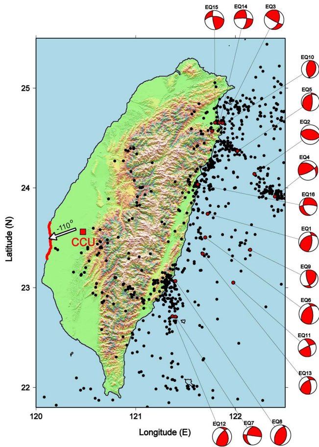
Fig. 1. Locations of epicentres and the CCU station. The black solid circles denote epicentres ( M \geq 4.0 ) from 2002 through 2005. The 16 earthquakes ( M \geq 5.5 ) in this study are represented by red solid circles. Fault plane solutions of earthquakes are shown in the map margin. The red rectangle indicates the CCU station. The red line is the coast line being close to CCU station.
