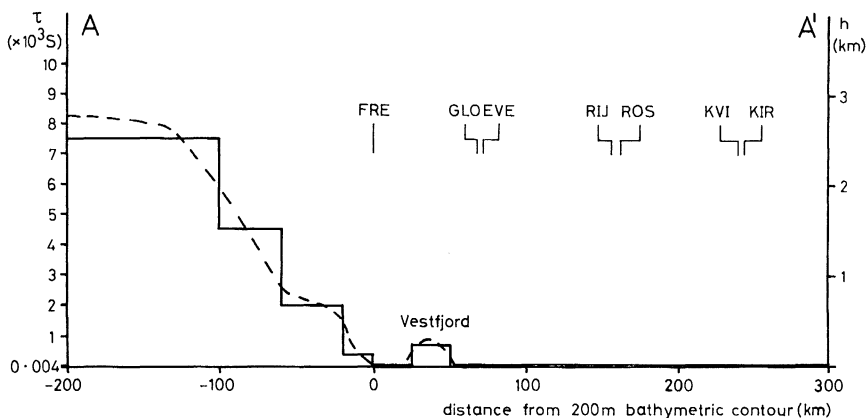
Fig. 14. Full line: thin-sheet model approximation of the lateral variation in crustal conductivity along Profile AA'. The continental crust has an integrated conductivity of 4 S. The locations of the stations, as resolved along AA', are also illustrated. The thin-sheet surface overlies a 110 km thick layer of 125 \Omega\text{m} , followed by a half-space of 3 \Omega\text{m} . Dashed line: the variation in bathymetry along profile AA'. The position of Vestfjord, which lies between the Lofoten Islands and the mainland, i.e., between FRE and GLO, is also indicated
