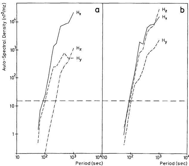
Fig. 8a, b. Smoothed Auto-Spectral Densities, in nT^2/Hz , for the data recorded at a KIR and b BER. H_x , H_y and H_z refer to the north, east, and vertical components respectively in the Kiruna system. The dotted line indicates the assessed resolution level (see text)
