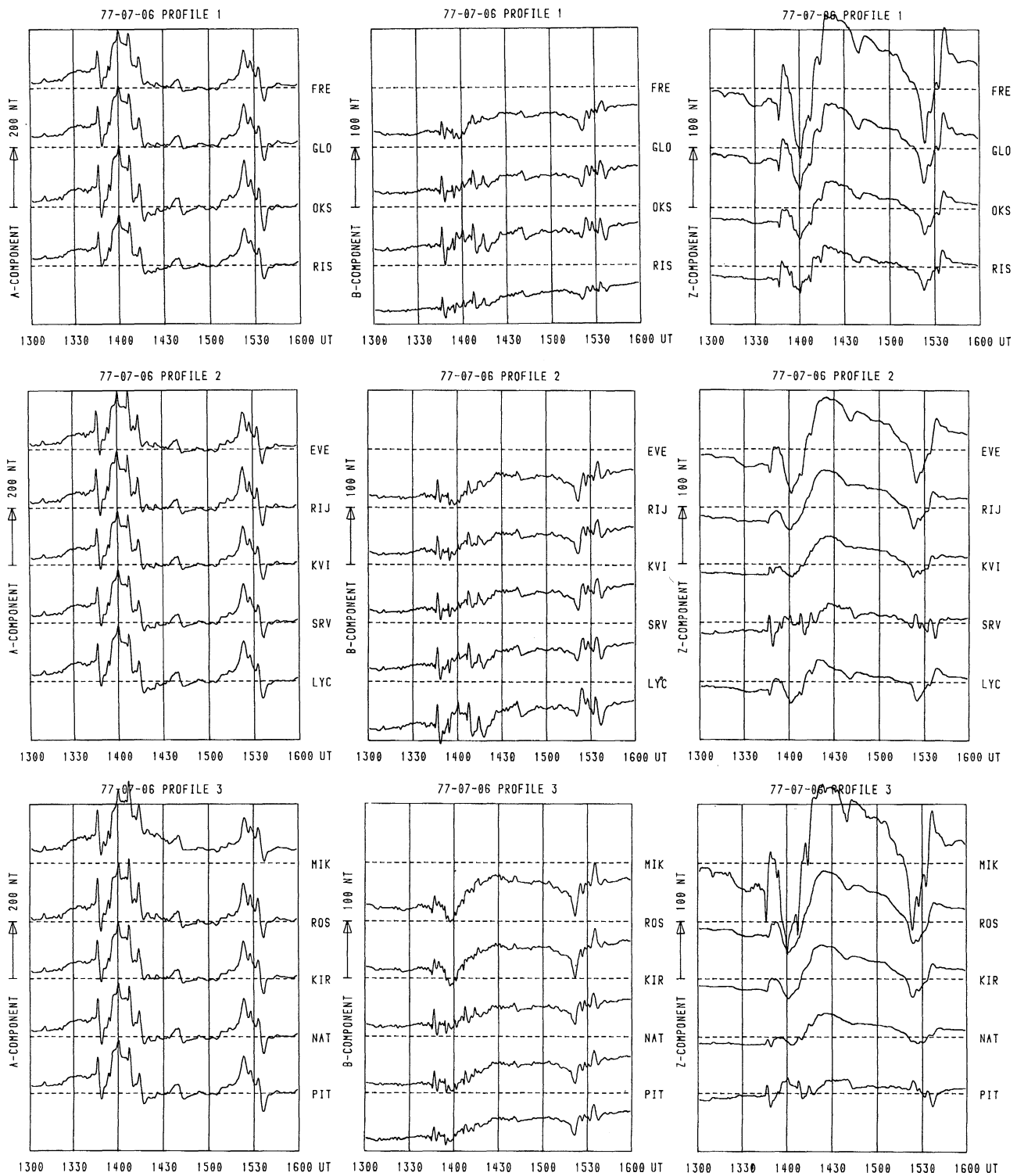
Fig. 2. Magnetic disturbances, as recorded by the stations illustrated in Fig. 1, in the interval 13:00–16:00 UT on 6 July 1977, compared with quiet-time baselines (dotted lines). A , B , and Z components refer to north, east, and vertical respectively in the Kiruna co-ordinate system (note: these components are termed x(t) , y(t) and z(t) in the text). The data are stacked along Profiles; Profile 1 FRE→RIS; Profile 2 EVE→LYC; Profile 3 MIK→PIT; Profile 4 SOY→SAU; Profile 6 BER→SKO
