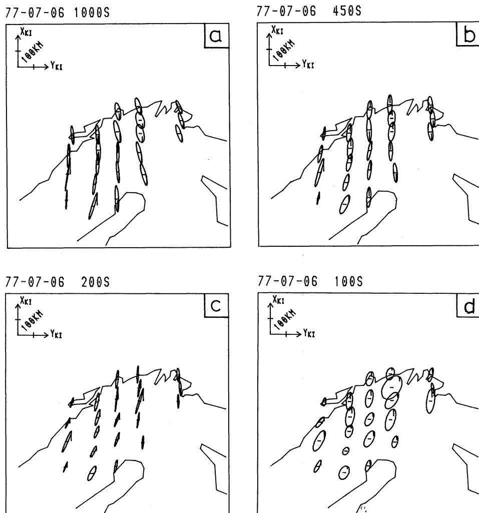
Fig. 9a-d. Ellipses of the polarised power of the horizontal magnetic field, as observed at a 1,000 s, b 450 s, c 200 s and d 100 s
