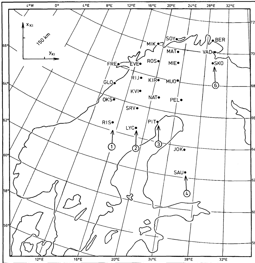
Fig. 1. Map showing the locations, in geographical co-ordinates, of the magnetometer stations which provided data for the event discussed in this study. In the upper left-hand corner are indicated the axes of the Kiruna cartesian co-ordinate system (see text). Profiles 1–4 and 6, which are perpendicular to lines of constant revised corrected geomagnetic latitude, are designated by the encircled numbers
