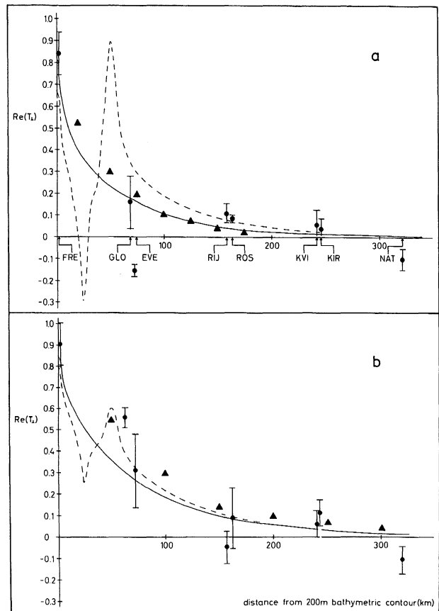
Fig. 13a, b. Dots indicate the magnitude of the real part of the inductive transfer function at a 200 s and b 1,000 s in the direction parallel to AA', i.e., perpendicular to the coast, or E-polarisation, for the stations FRE, GLO, EVE, RIJ, ROS, KVI, KIR, and NAT, as compared to the distance from the 200 m bathymetric contour west of FRE (see Fig. 12). The ranges are the 68 % confidence intervals of the rotated functions. Triangles indicate the Fischer first-approximation of a perfectly conducting thin sheet overlying a half space at a 200 s and b 1,000 s for half-spaces of 230 \Omega\text{m} and 130 \Omega\text{m} respectively. Full lines are the Schmucker thin-sheet modelling results for the model shown in Fig. 14 without a Vestfjord representation. Dashed lines are the Schmucker thin-sheet modelling results for the model shown in Fig. 14 with a tau representation of Vestfjord (see text)
