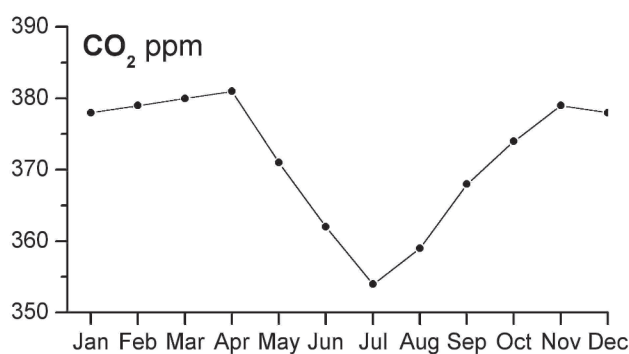
Figure 4. Seasonal variations of carbon dioxide concentrations near Tomsk.
