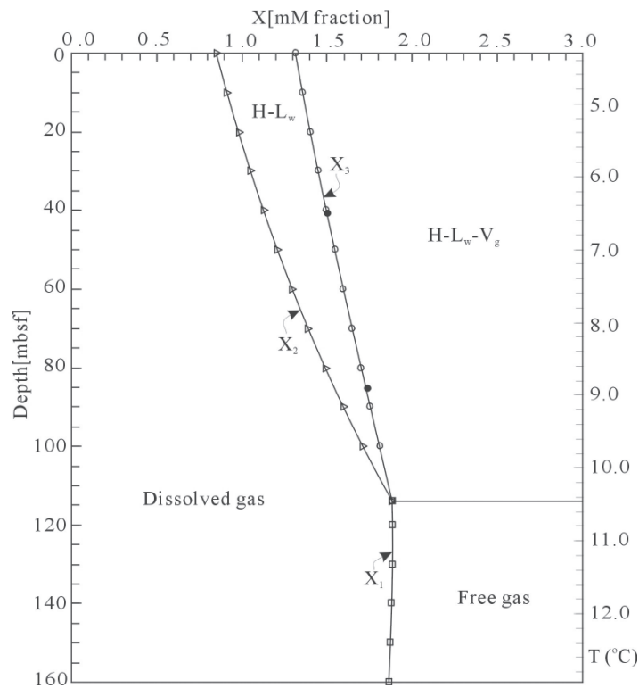
Fig. 4. Equilibrium solubility of methane at site 1249 in the southern summit of Hydrate Ridge. H - L w is hydrate-water system, and H - L w - V g is hydrate-water-free gas system. Black dots are measured data from Servio and Englezos (2002) and is consistent with our calculated phase curve of hydrate-gas-seawater system.
