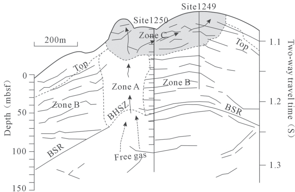
Fig. 1. Schematic illustration of gas hydrate occurrence across the southern summit of Hydrate Ridge (after Trehu et al. 2004). BHSZ is the base of the hydrate stability zone. Zone C and possibly zone A are a three-phase hydrate system, while zone B is a two-phase hydrate system. Arrows show the route of gas venting. Vent gas from a free gas zone under BSR may migrate to zone C through zone A where is a wipeout zone in seismic profile.
