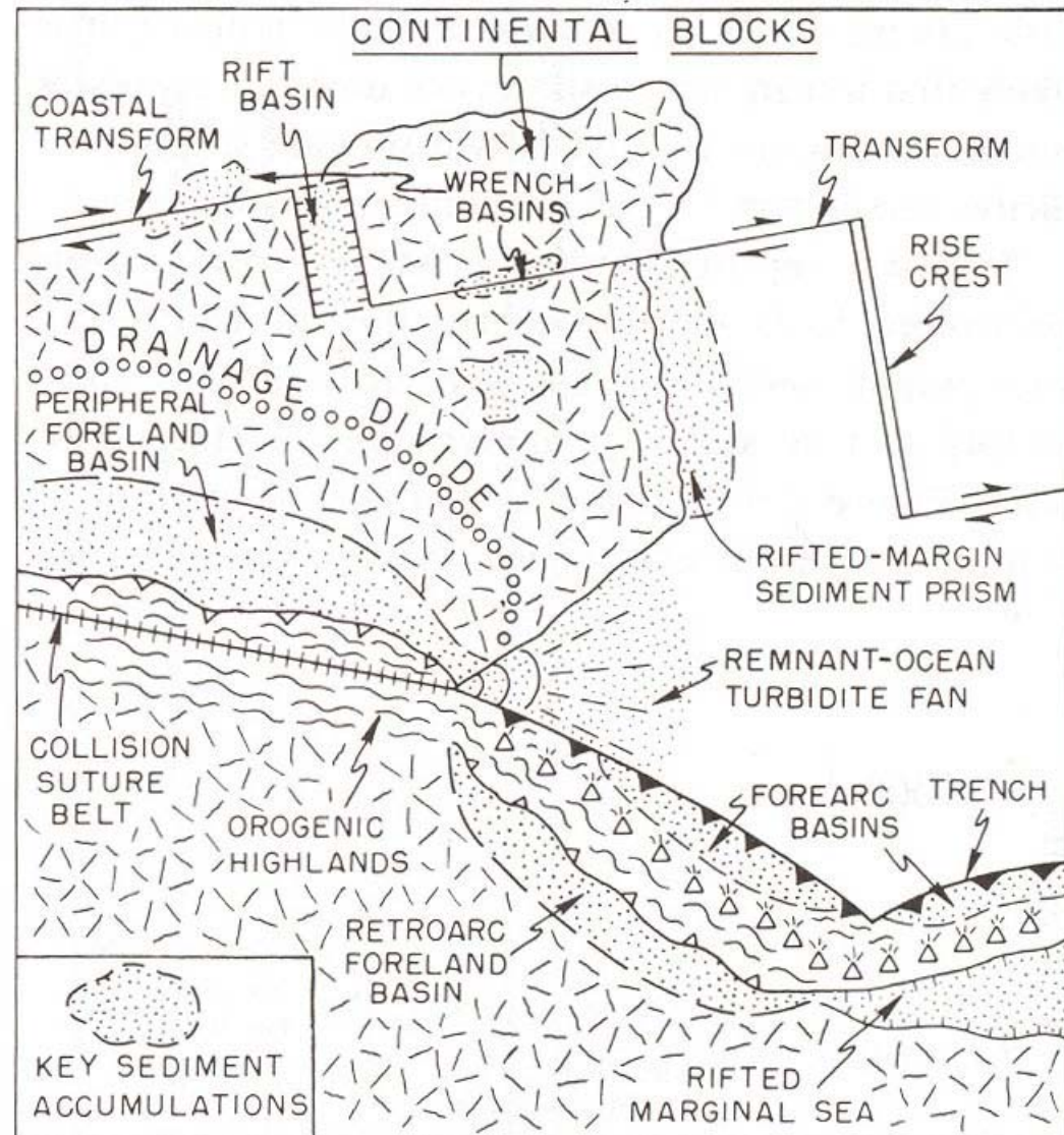
Sites of key basins in relation to plate boundaries, continental margins and associated sources of detrital sediment (Busby & Ingersoll, 1995)
