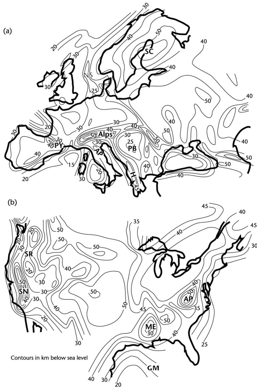
Fig. 1.2 Depth to the Moho below sea-level from (a) Europe and (b) North America, after Allenby and Schnezler (1983) and Meissner (1986). In Europe, thick continental crust occurs in the Pyrenean-Alpine-Carpathian orogenic belt and in the Scandinavian Shield. Thin continental crust occurs along the Atlantic margin and in regions of continental stretching , such as the North Sea, western Mediterranean, Pannonian Basin, and Black Sea. In North American, thick continental crust is associated with the batholiths of the Sierra Nevada region, the Appalachian orogenic belt, the American midcontinent and the Canadian-NE USA shield. Thin crust is associated with the plateau basalts of the Snake River area, sites of rifting such as the Mississippi Embayment, and along the western active continental margin, eastern passive continental margin and the Gulf of Mexico. NS, North Sea; SC, Scandinavian Shield; PY, Pyrenees; AP, Apennines; PB, Pannonian Basin; H, Hellenides; SR, Snake River; SN, Sierra Nevada; ME, Mississippi Embayment; AP, Appalachians; GM, Gulf of Mexico.
