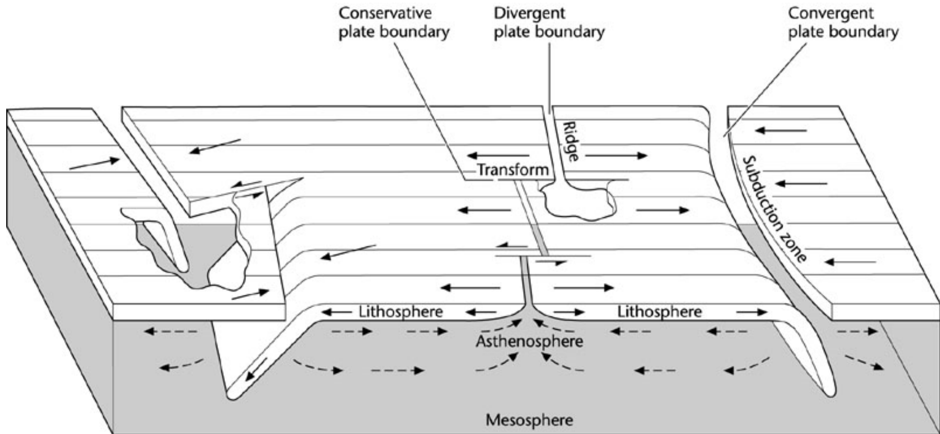
Fig. 1.6 The three types of plate boundary: convergent, divergent, and conservative.
