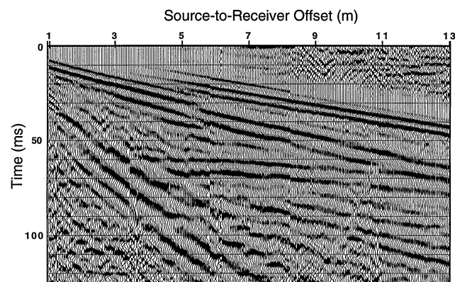
FIG. 3. Pseudowalkaway field file for the .22-rifle source, without board-mounted geophones, displayed with a 25-ms automatic gain control (AGC) window and a band-pass filter from 300 to 400 Hz with 12 dB/octave slopes. The receiver interval is 5 cm. The prominent reflection at 60 ms is from either a clay-sand interface at a depth of about 9 m or the water table within the clay at about 8 m. The bedrock reflection at this site exhibits a very strong amplitude-variation-with-offset effect; as a result, the bedrock reflection often is not obvious on field records at offsets of less than 15 m.
