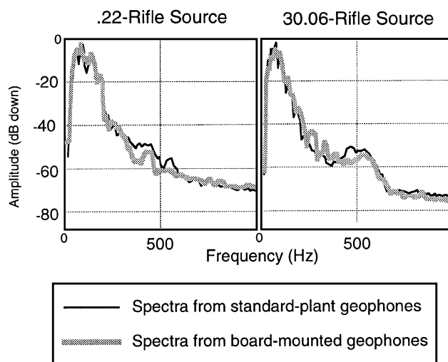
FIG. 11. Comparison of frequency spectra for the .22- and 30.06-rifle sources for board-mounted versus standard-plant geophones. In each case, the spectra were averaged over the 12 traces shown in Figures 9 and 10.
