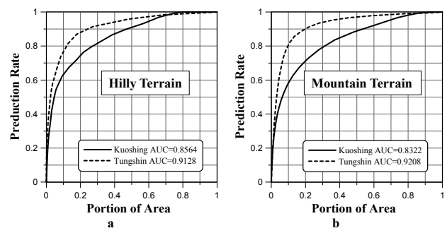
Fig. 13. Prediction rate curve for a subsequent event – the typhoon Mindulle, in the Kuohsing and Tungshih quadrangles. (a) Hilly terrain, (b) mountainous terrain. AUCs are indicated.
