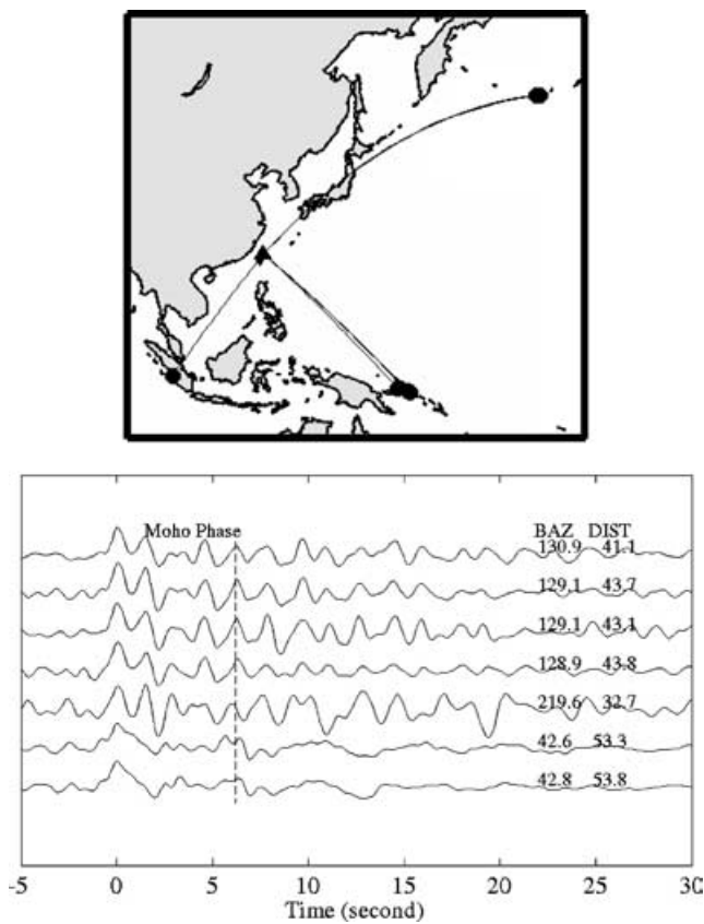
Figure 14. (a) Examples of radial-component receiver functions for NACB station north of the suture zone between the Philippine Sea and the Eurasian plates showing similar receiver function waveforms for earthquakes from all directions except the northeast direction. (b) Inversion results for NACB station are shown with the same format as in Fig. 7. The preferred Moho depth is around 50–52 km.
