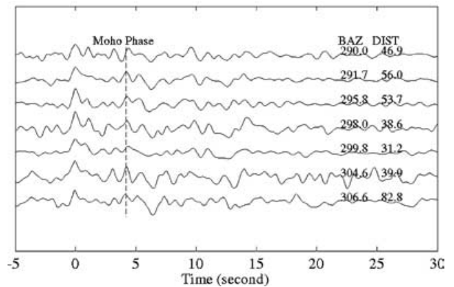
Figure 11. (a) Examples of radial-component receiver functions for TPUB station in southwestern Taiwan showing similar receiver function waveforms for earthquakes from the west. (b) Inversion results for TPUB station are shown with the same format as in Fig. 7. A mid-crust discontinuity can be identified at depth \sim 20 km which can be interpreted as the Conrad discontinuity. The preferred Moho depth is around 30–32 km.
