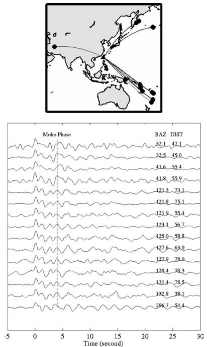
Figure 8. (a) Examples of radial-component receiver functions for TWKB station in southern Taiwan showing very similar receiver function waveforms for earthquakes from all directions. (b) The inversion result for TWKB station is shown with the same format as in Fig. 7. The preferred Moho depth is around 30–32 km.
