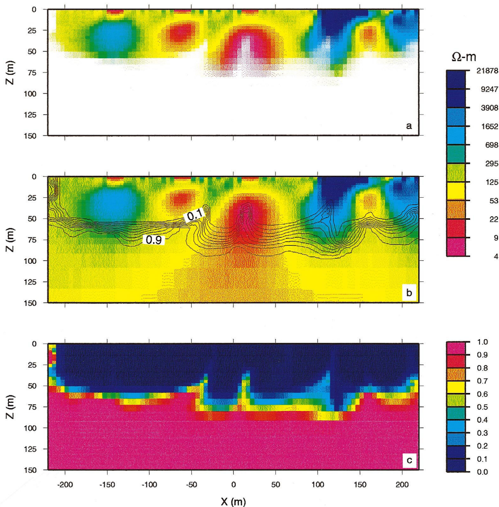
FIG. 6. The DOI index computed from inversions using ramp reference models is plotted in (c). These values are superposed on m^* in (b). The contour interval is 0.1. In (a) the intensity of m^* is scaled by the DOI value.
