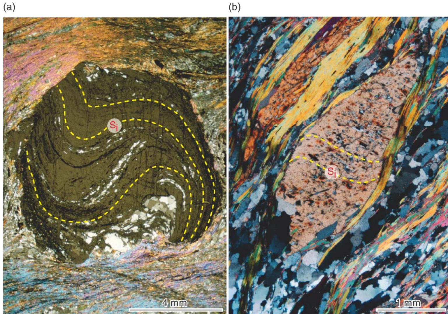
Figure 21.2 (a) Garnet porphyroblast in micaschist, showing sigmoidal pattern. The inclusion pattern is an earlier foliation now disconnected and at high angle to the external foliation. (b) Amphibole porphyroblast with (mostly) straight inclusion trails. Straight trails may indicate pre- or intertectonic growth, but the curvature close to the boundary may indicate that deformation initiated during the last part of the growth history.
