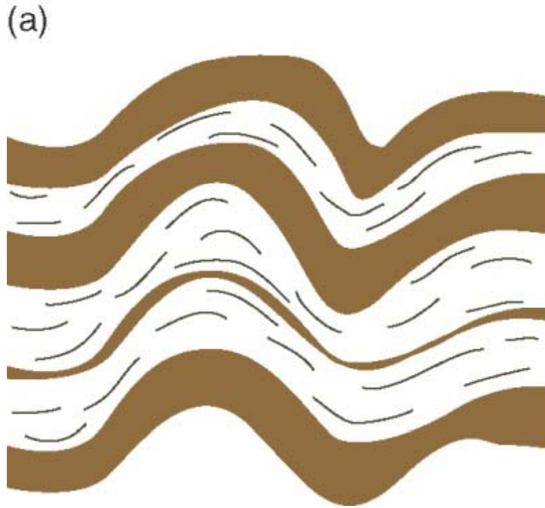
Figure 12.22 Schematic illustration of transposition by horizontal shortening and vertical extension. Both coaxial and non-coaxial strain can produce this result. The result (b) is a banded rock with intrafolial folds and isolated fold hinges. Note how the dominant foliation changes (transposes) from horizontal (a) to vertical (b).
