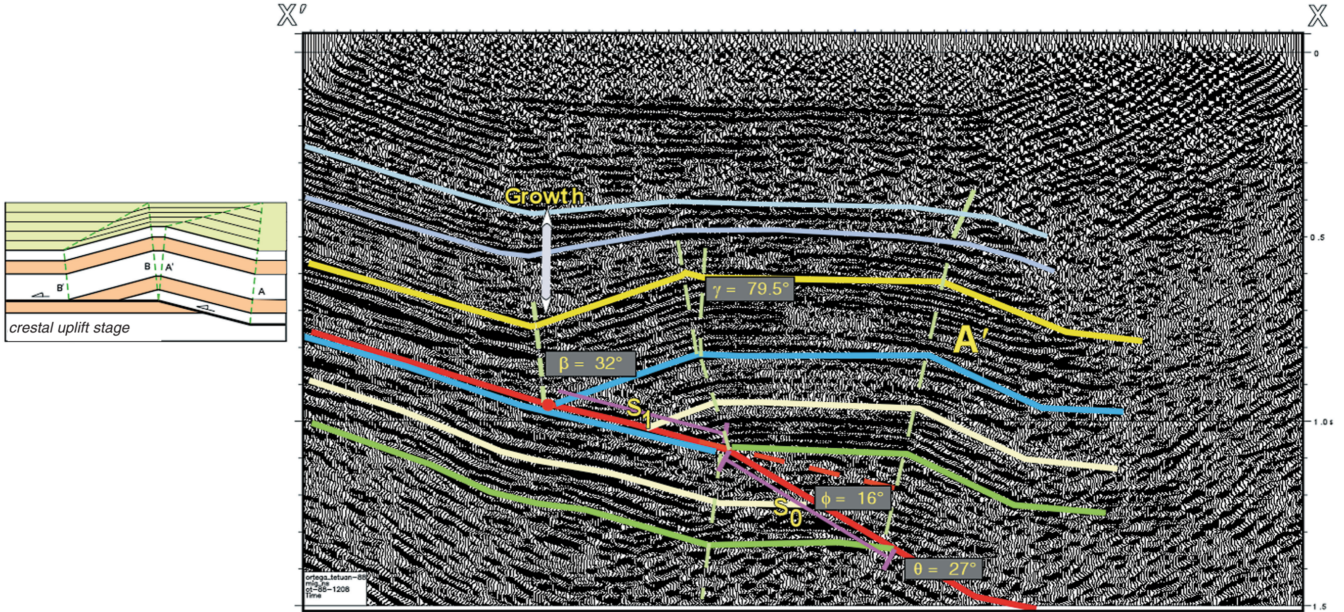
Seismic Interpretation of Contractional Fault-Related Folds An AAPG Seismic Atlas
