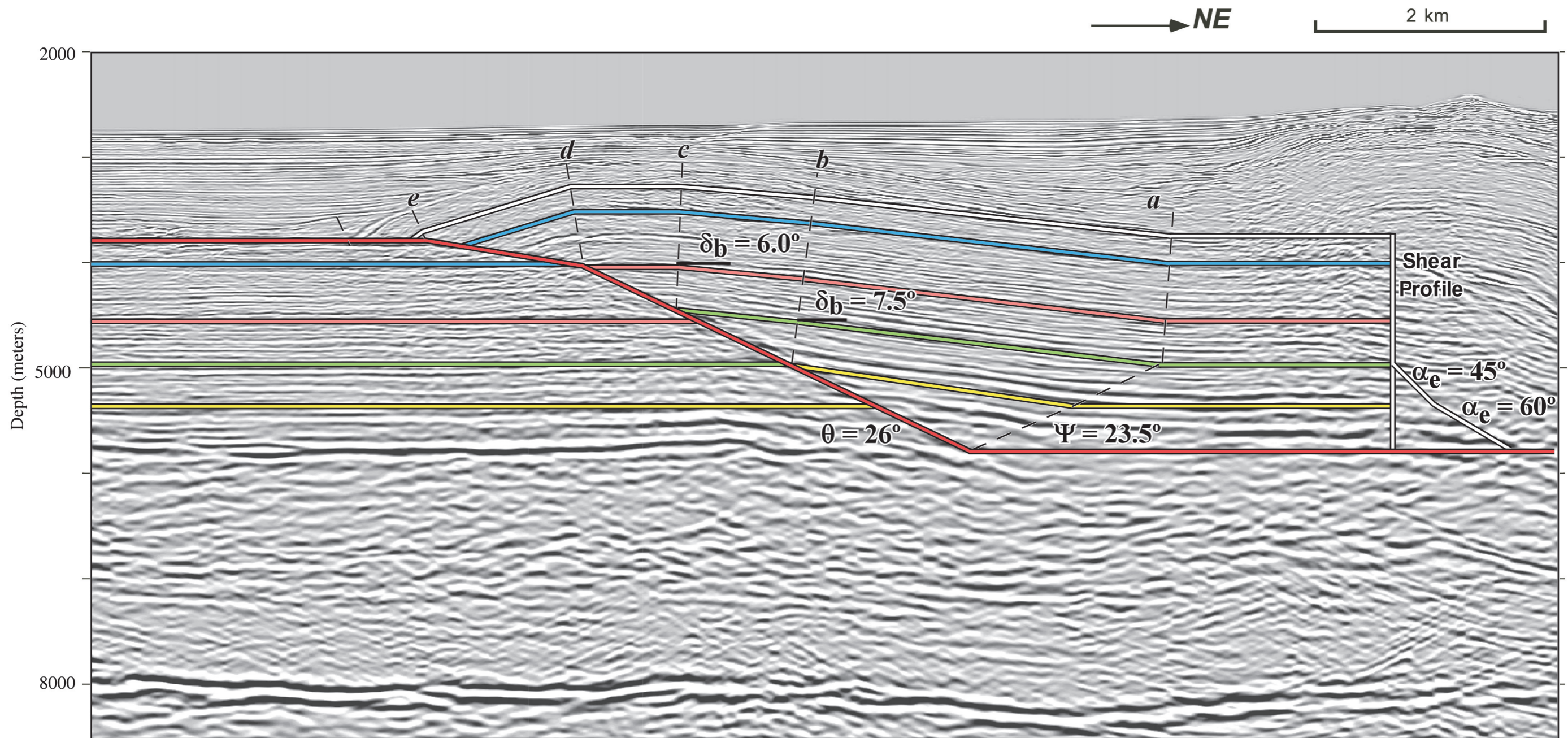
Pure Shear Fault-bend Fold
