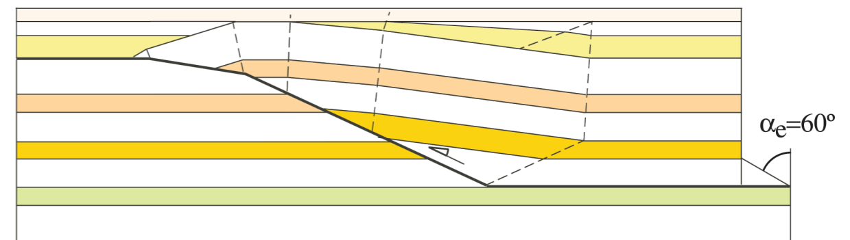
Pure Shear Fault-bend Fold
