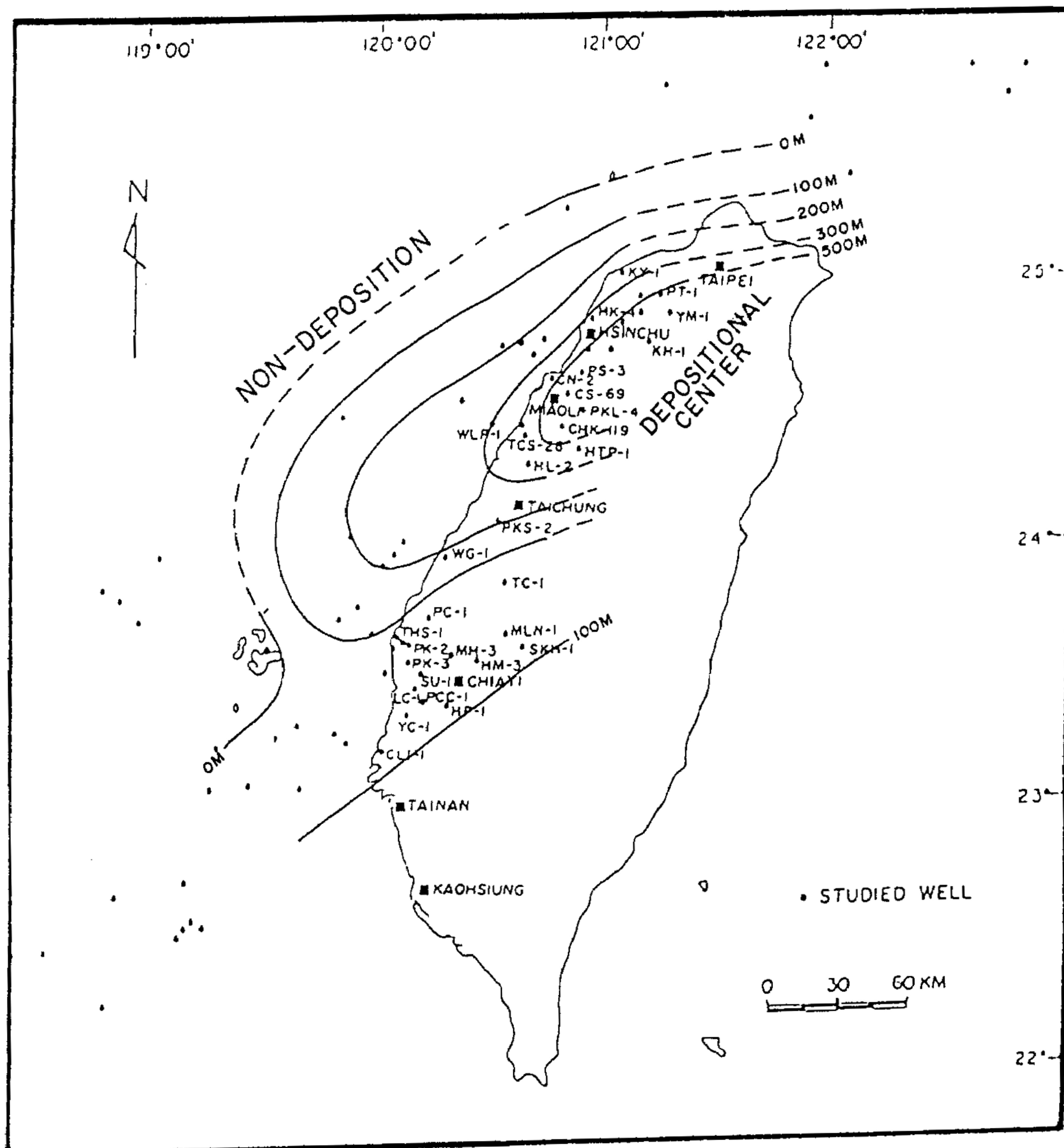
Fig. 12. Isopach map of the Shihti Formation, Western Taiwan Basin.
