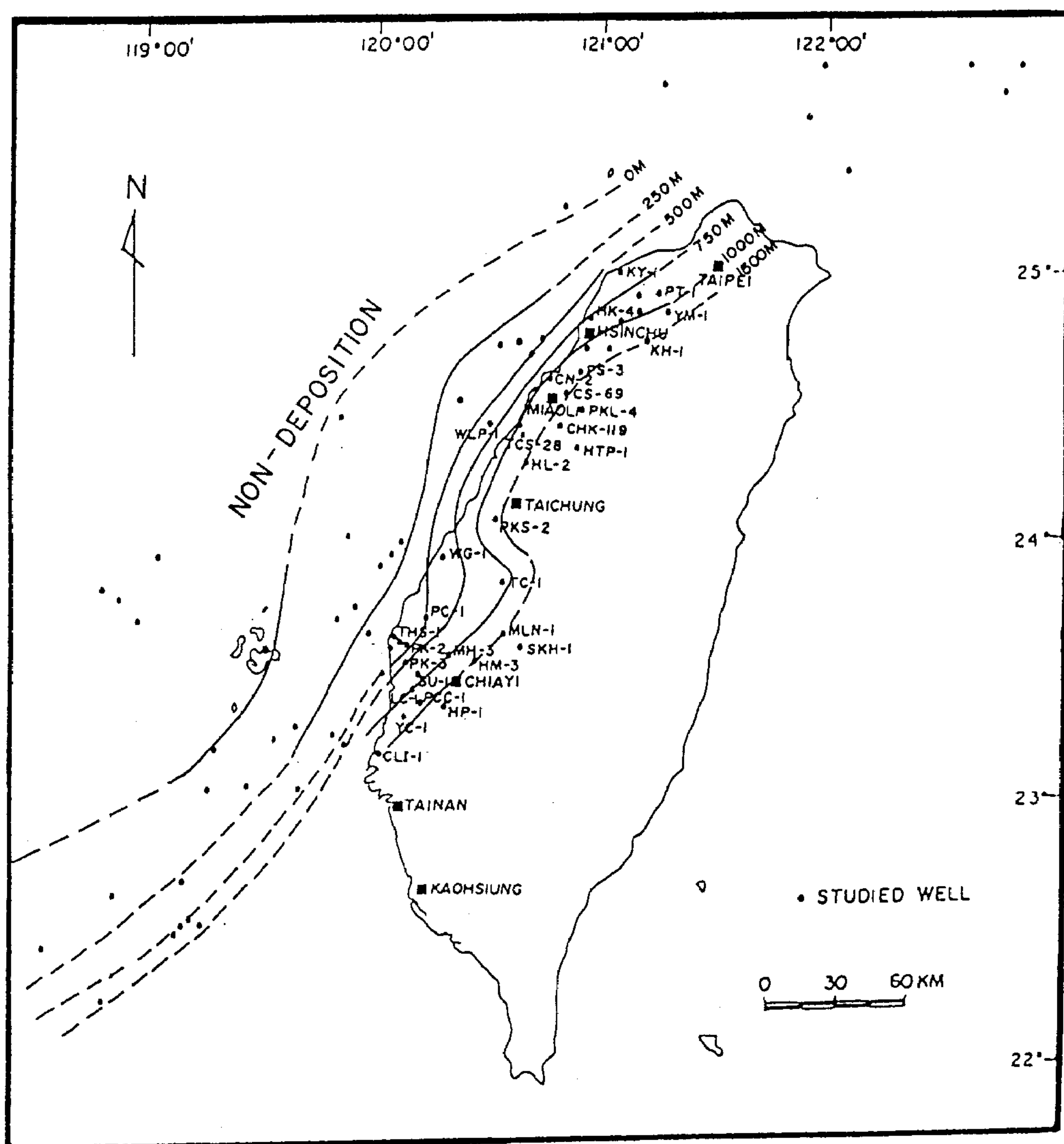
Fig. 18. Isopach map of the Cholan Formation, Western Taiwan Basin.
