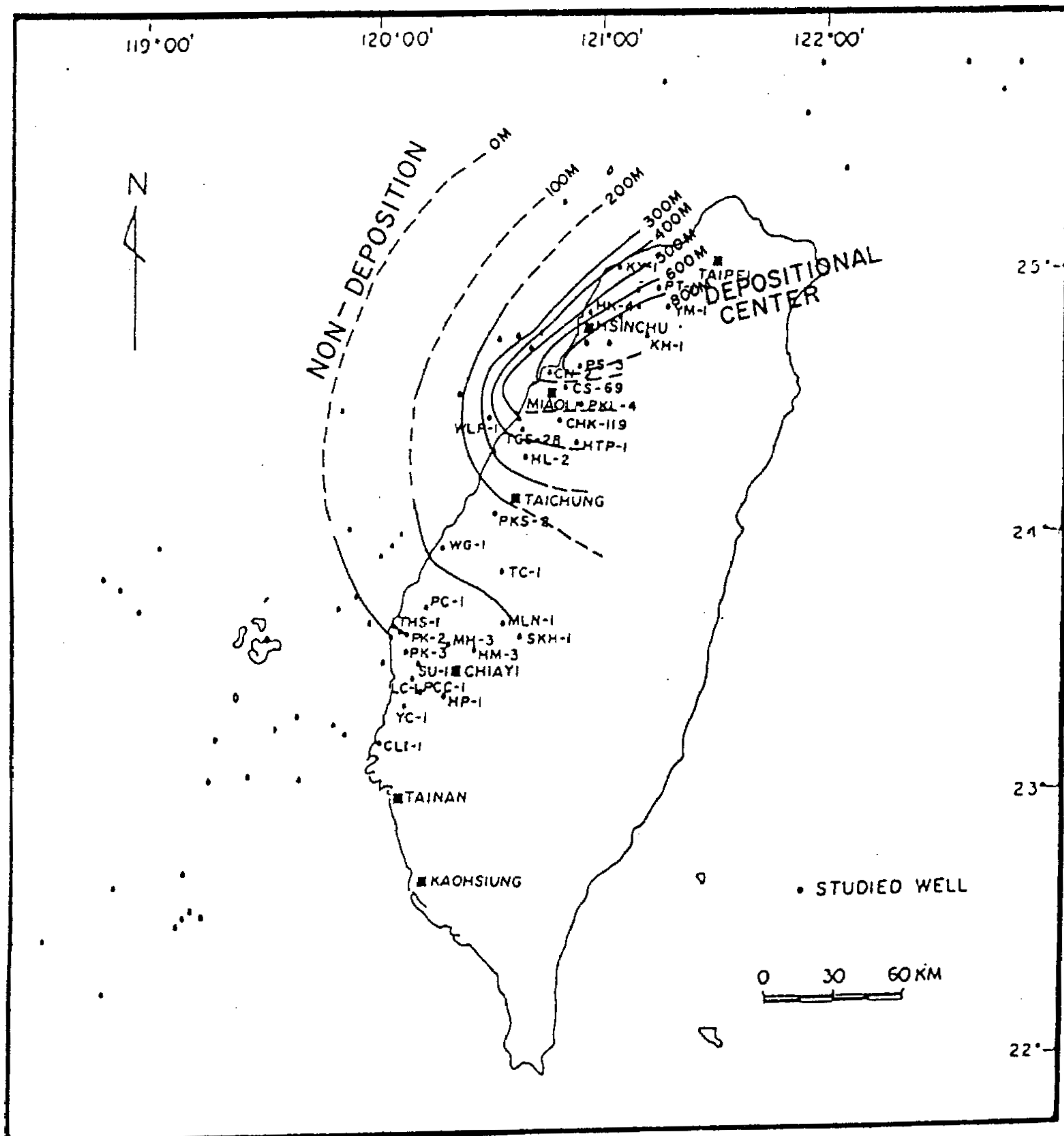
Fig. 16. Isopach map of the Kueichulin Formation, Western Taiwan Basin.
