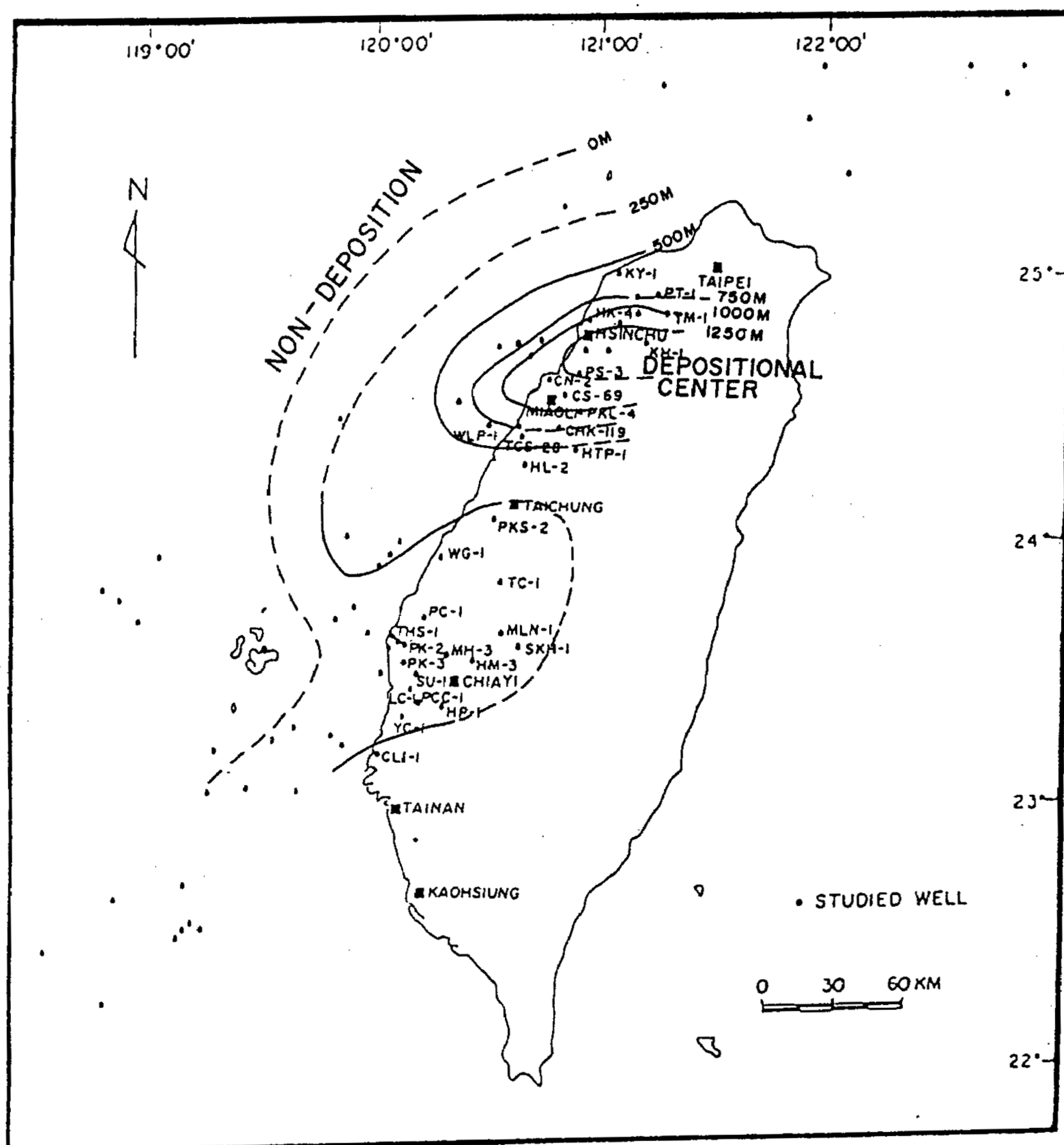
Fig. 15. Isopach map of the Kuanyinshan Sandstone and Nanchuang Formation, Western Taiwan Basin.
