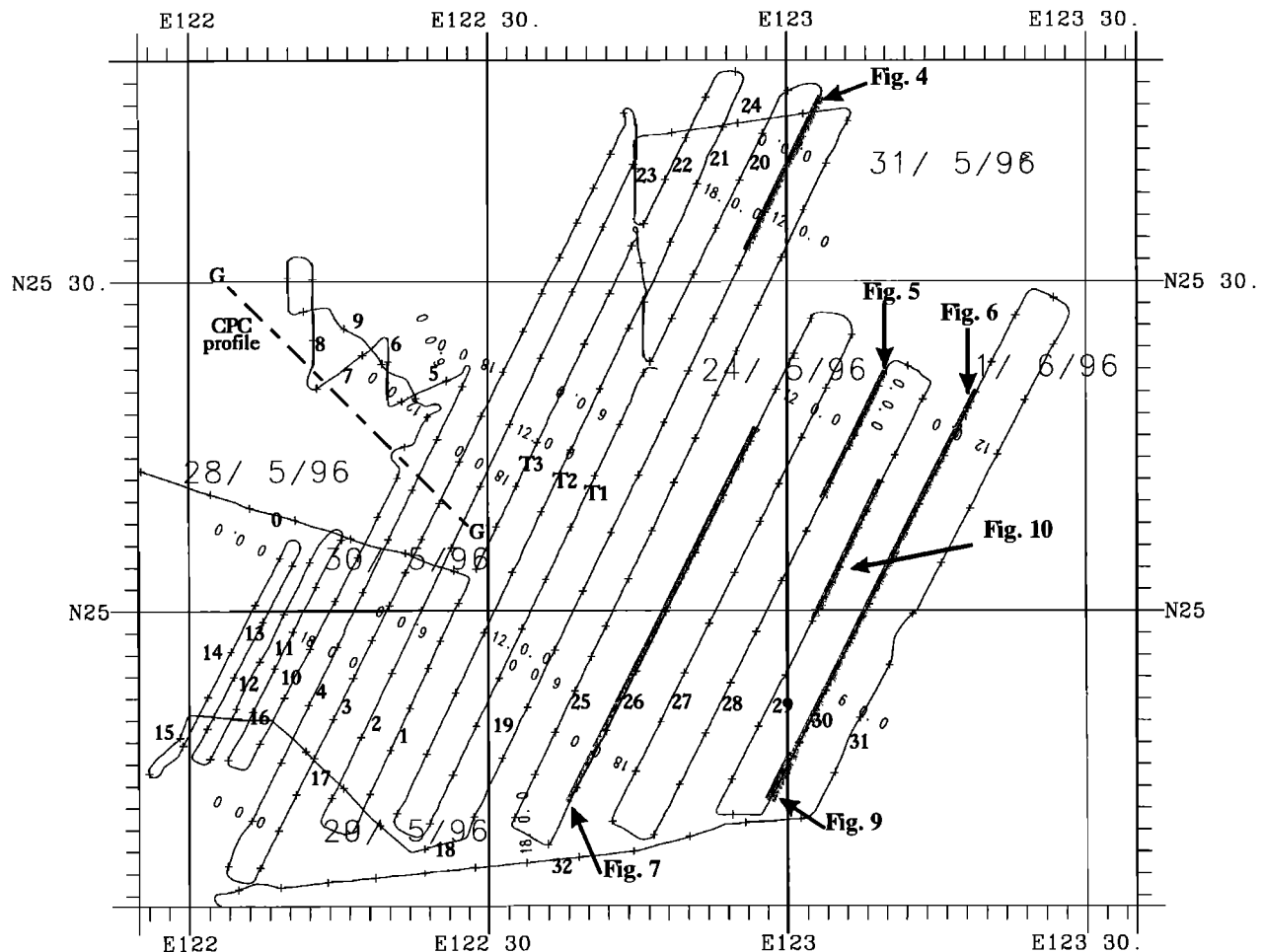
Figure 2. Track lines of the ACT cruise and the preceding transit of the R/V l'Atalante (May-June 1996) in the southwestern Okinawa Trough with locations of portions of profiles displayed in the following figures. GG', Chinese Petroleum Company seismic profile [Huang et al. , 1992].
