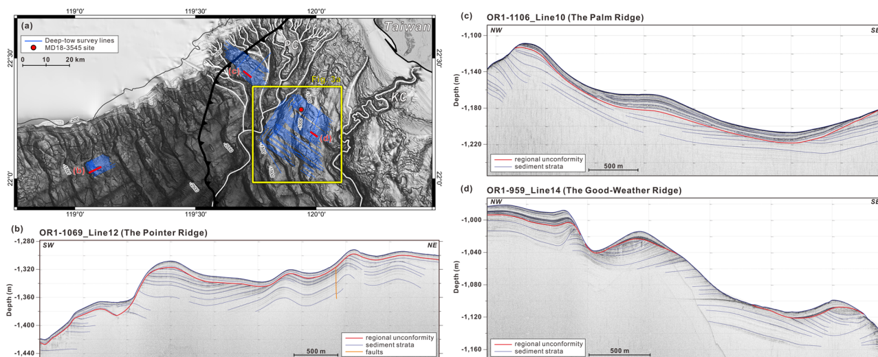
Fig. 2 | The sub-bottom profiler data and the regional unconformity in the continental slope of the NE South China Sea. a Blue lines indicate the deep-tow survey lines. A regional unconformity could be recognized in the continental slopes shown in the sub-bottom profiler (SBP) data of (b), (c) and (d). A red dot indicates
