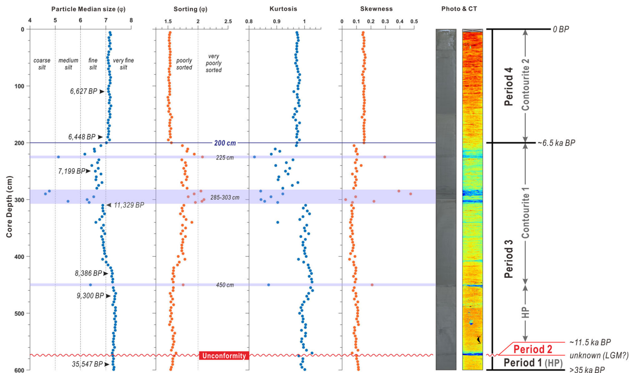
Fig. 4 | The analysis results of the top 600 cm of core MD18-3545. The charts from left to right are particle median size, sorting, kurtosis, skewness, core photo and CT image, respectively. Based on the core analysis results, we could distinguish four sedimentary periods and sediment facies in each period. The black arrows with age
