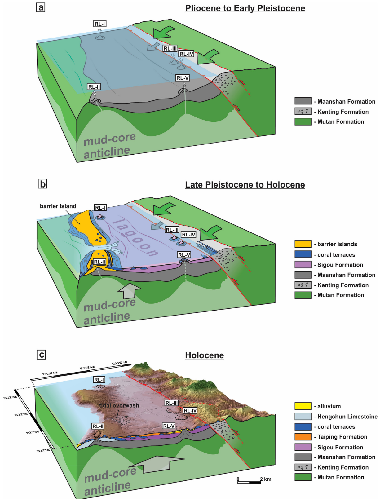
Fig. 15. Evolutionary model of the trench-slope basin of the southwestern Hengchun Peninsula. (a) Trench-slope basin stage. Rapid sedimentation from erosion emerged the Mutan Formation and Kenting Mélange by depositing material with large amounts of organic matter. The overpressure of the produced gas hydrates leads to mud diapirism; (b) lagoon stage. An emerging basin changes the environment to warmer and shallow water. Sediment of the same source then fills the already lagoonal basin blocked by barrier islands to the west; (c) onshore stage. The emerged basin exposes landforms of preexisting mud volcanoes and lagoonal features as tidal overwash, barrier islands. However, continuous erosion progressively erodes the mud volcanoes leaving oval-shaped relicts covered by more resistant coral terraces. Alluvial deposits cover the lagoon, though the deformation of the basin still remains active.
